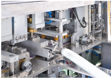
Punching hole
