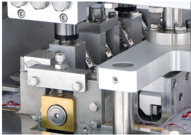
Cutting length
