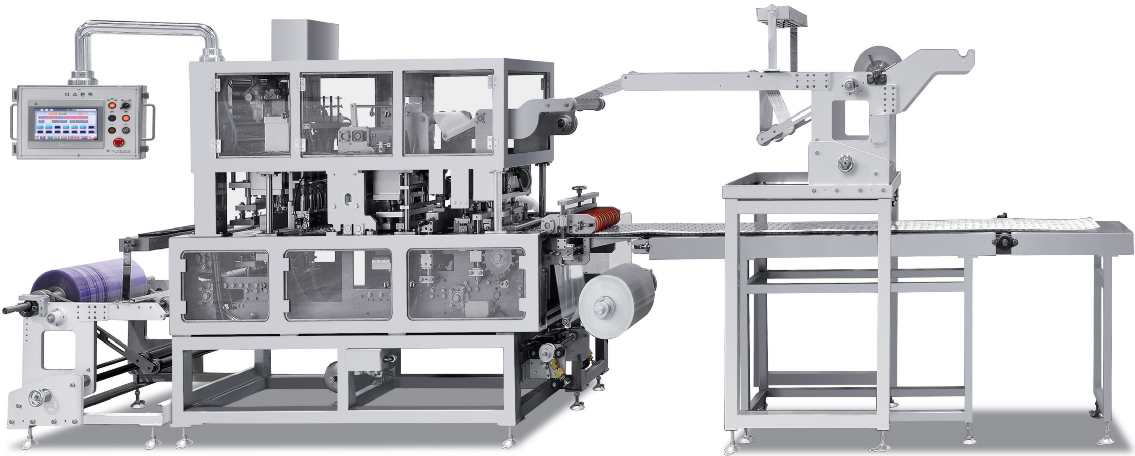
Sealing
