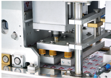
Sealing
